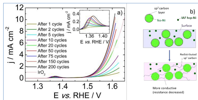
Fig. 7 a) Polarization curves recorded at 5 mV s -1 after different numbers of voltammetric cycles in nitrogen saturated 1 M KOH electrolyte, b) Schematic showing removal of the carbon shell surrounding fcc-Ni particles to be redistributed within the Si-C-O-N(H) matrix under working conditions in a 1 M KOH electrolyte.
