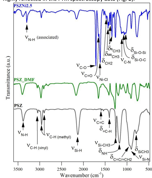
Fig. 2 FTIR spectra of the PSZNi2.5_5 , PSZ and PSZ_DMF samples.
