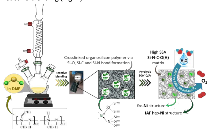
Fig. 1 Schematic diagram of the two-step general process of designing Si-C-O-N(H) immobilized nanoscaled Ni pre-catalysts.
