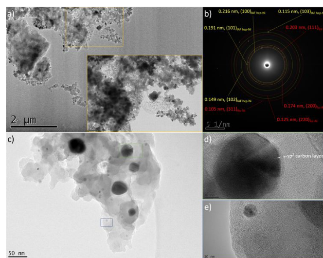
Fig. 6 Low magnification TEM images of the PSZNi2.5_5 sample (a-c), SAED pattern corresponding to image a) (b) and high magnification images of nanoparticles isolated in the PSZNi2.5_5 (d-e).
