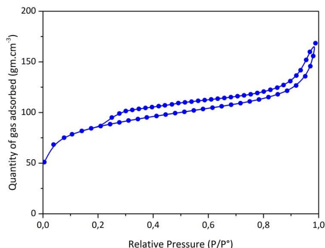
Fig. 3 \text{N}_2 sorption isotherms of the PSZNi2.5_5 sample.
