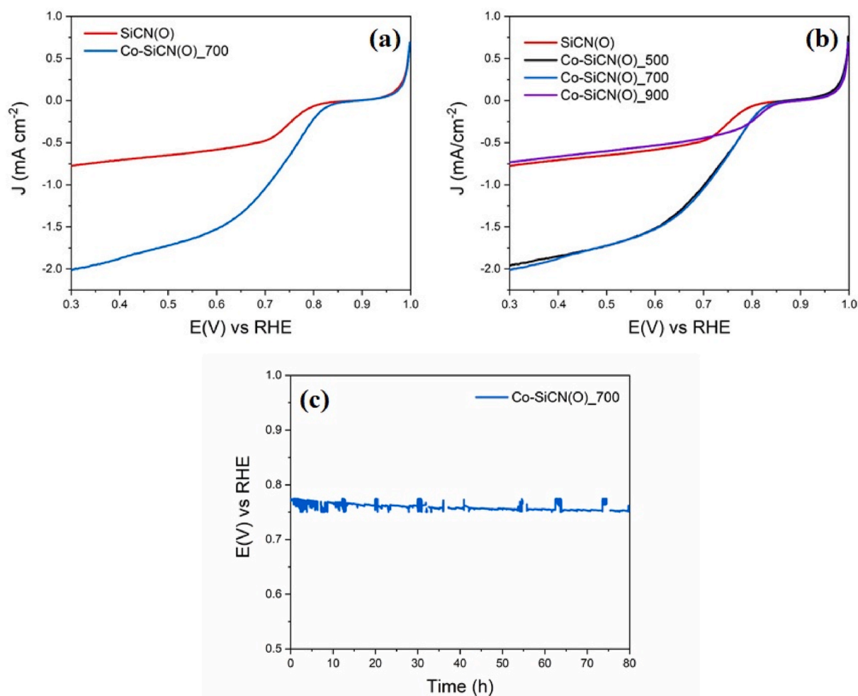
Fig. 8. Electrochemical activity of prepared catalysts towards ORR: (a) LSV of SiCN(O) and Co-SiCN(O)_700, (b) dependence on pyrolysis temperature and (c) Chronopotentiometric stability test performed at 10 \text{ mA cm}^{-2} for 80 h.
